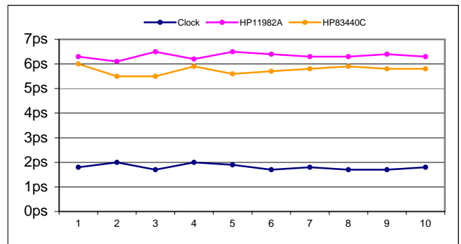
Fig.5 - Three sets of 10 jitter measurements made in the laboratory.
