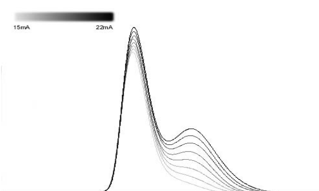
Fig. 8 – Evolution of the timing jitter when the laser drive current increases.
