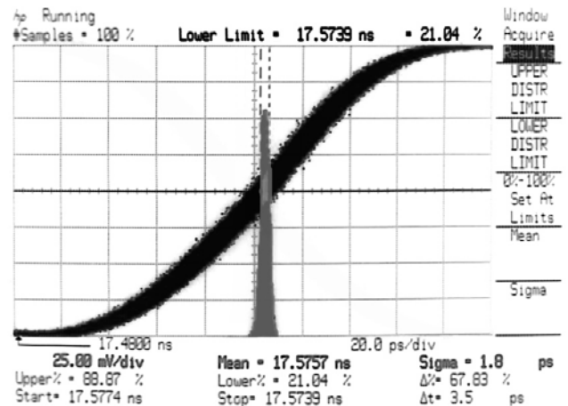
Fig.4 - Photograph of an histogram of a temporal portion of an eye diagram obtained on the oscilloscope. The signal being analysed is the clock signal.
