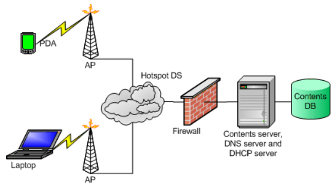
Figura 5 - Architecture to an open access hotspot without Internet access
