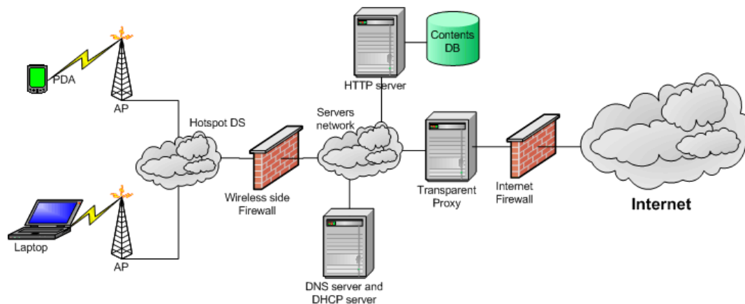
Figura 4 - Architecture to an open access hotspot with Internet access
