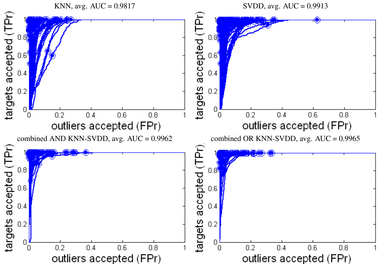
Fig. 7 - ROC of the 70 individual classifiers and their average AUC for each type of OCC considered and using feature trios.
