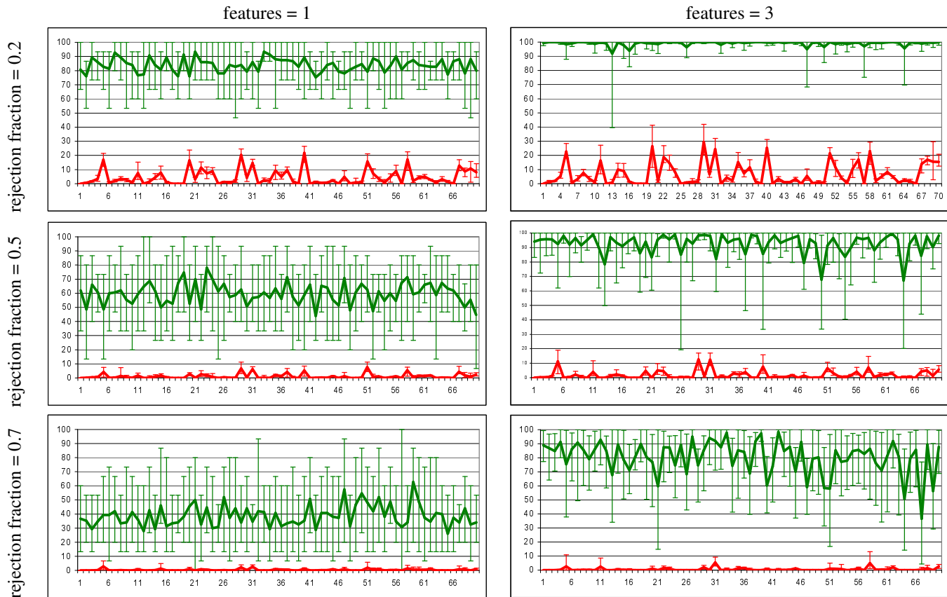
Fig. 6 - Average individual classification results of the combined OR KNN-SVDD classifier, obtained after 10 independent tests. The upper (green) curve in each graphic shows the average correct owner classifications per classifier, while the lower (red) curve shows the average false positives per classifier. The vertical line under each average value shows the maximum and minimum values observed in the 10 tests.
