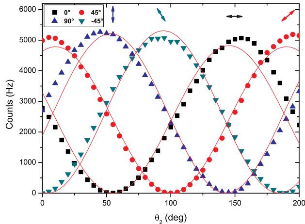
Fig. 2 - Average number of counts (Hz) as a function of the angle \theta_2 (degrees), for the linear SOPs with angles \theta_1 = 0, 45, 90 and -45 degrees, for back-to-back. \theta_1 is the angle of the single-photon source, and \theta_2 is the angle of the analyzer. The pump and signal optical powers at the fiber input were P_1 = 2.20 mW, and P_2 = 0.69 mW, respectively. The wavelengths for the pump and the signal were \lambda_1 = 1549.32 nm and \lambda_2 = 1550.92 nm, respectively. The theoretical fits given by (7) are represented by the solid lines.
