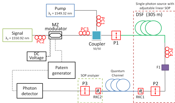
Fig. 1 - Experimental setup used to generate and detect single photons at the linear SOPs with angles 0, 45, 90 and -45 degrees. Details of the setup are presented in the text.
