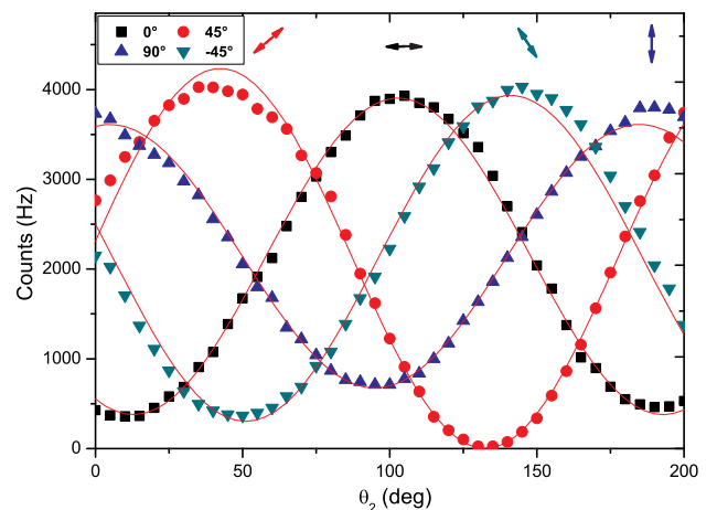
Fig. 4 - Average number of counts (Hz) as a function of the angle \theta_2 (degrees), for the linear SOPs with angles \theta_1 = 0, 45, 90 and -45 degrees, using a SMF with a length equal to 10 m, as a quantum channel. \theta_1 is the angle of the single-photon source, and \theta_2 is the angle of the analyzer. The optical powers and the wavelengths are the same used in Fig. 2. The theoretical fits given by (7) are represented by the solid lines.
