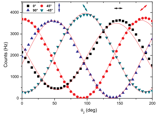
Fig. 3 - Average number of counts (Hz) as a function of the angle \theta_2 (degrees), for the linear SOPs with angles \theta_1 = 0, 45, 90 and -45 degrees, using a SMF with a length equal to 1 m, as a quantum channel. \theta_1 is the angle of the single-photon source, and \theta_2 is the angle of the analyzer. The pump and signal optical powers at the fiber input were P_1 = 2.07 mW, and P_2 = 0.61 mW, respectively. The wavelengths are the same used in Fig. 2. The theoretical fits given by (7) are represented by the solid lines.
